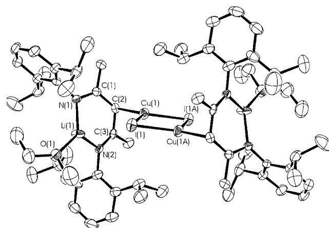
Figure 4. Crystal structure of 4 (hydrogen atoms are omitted for clarity)
