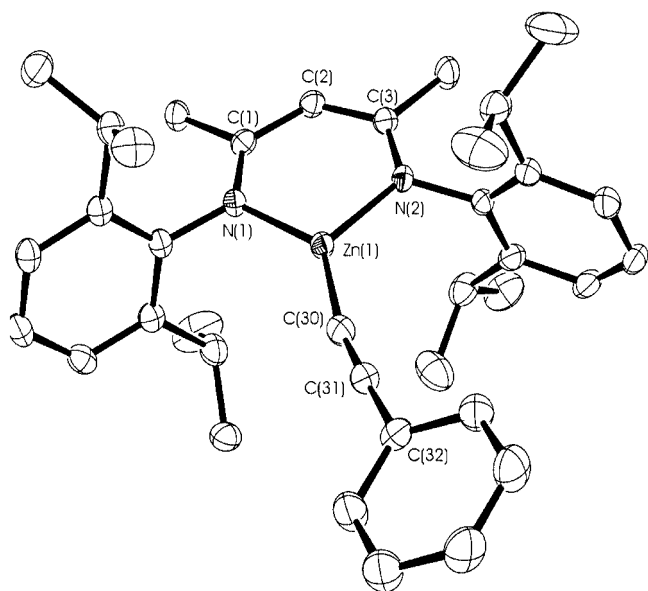
Figure 2. Crystal structure of 2 (hydrogen atoms are omitted for clarity)
