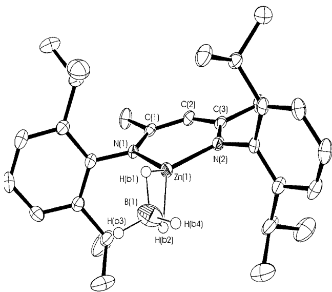
Figure 3. Crystal structure of 3 (hydrogen atoms are omitted for clarity)
