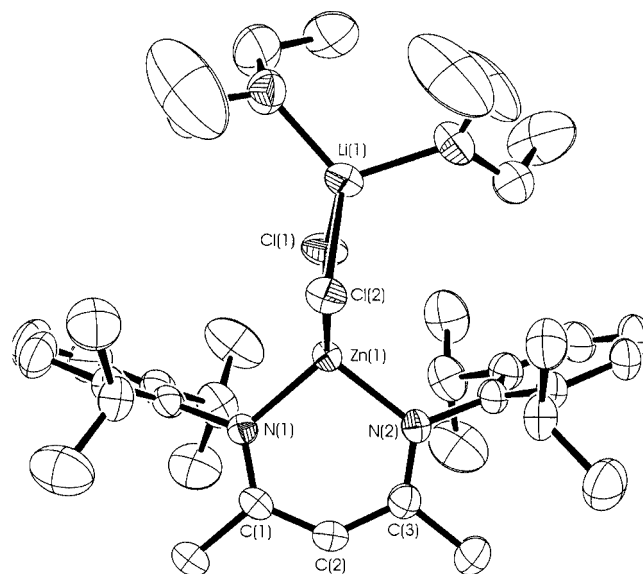
Figure 1. Crystal structure of 1a (hydrogen atoms are omitted for clarity)
